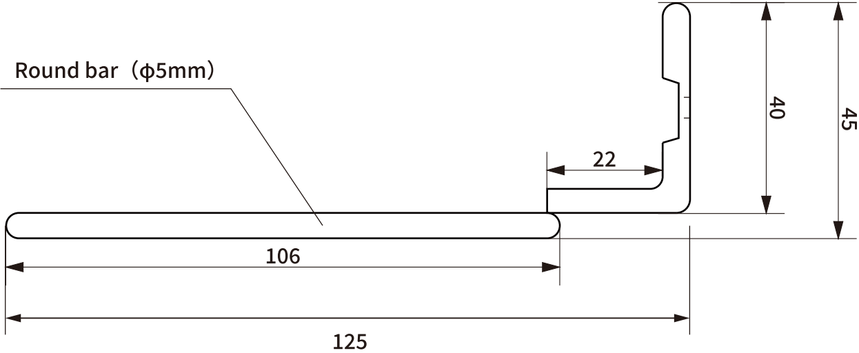
● Side view
