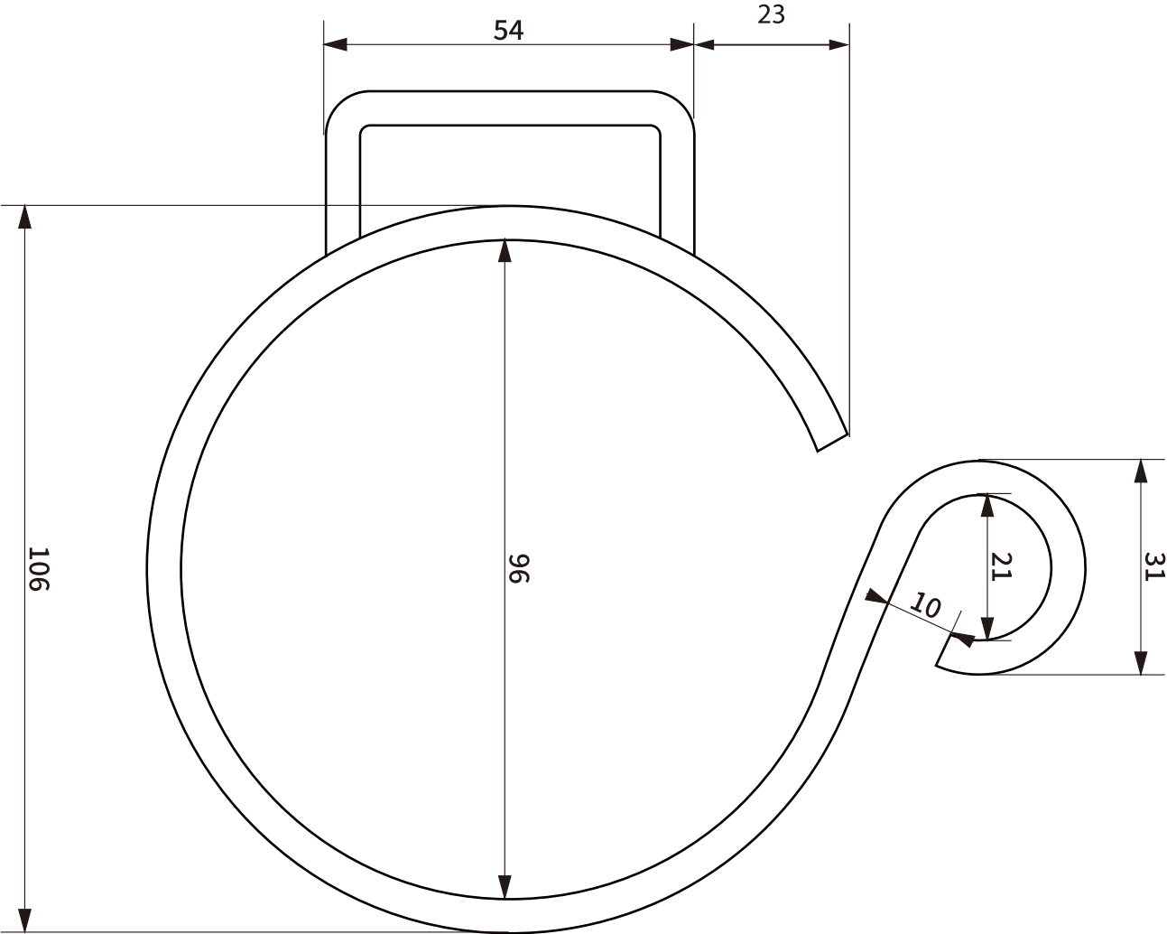
● Top view
