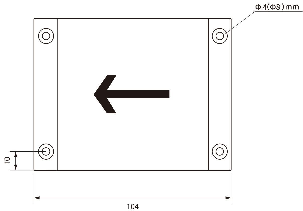
●Front view
