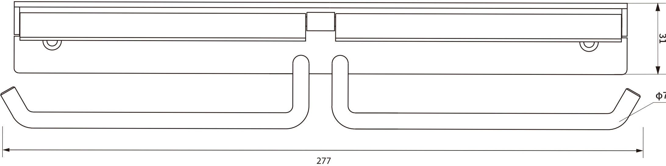
● Front view
