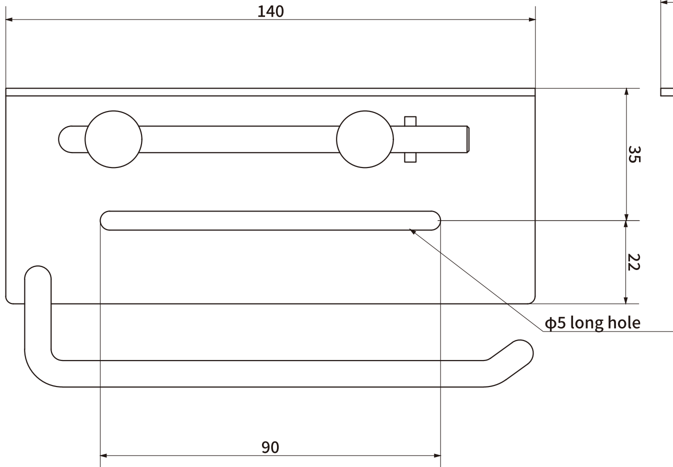
● Front view
