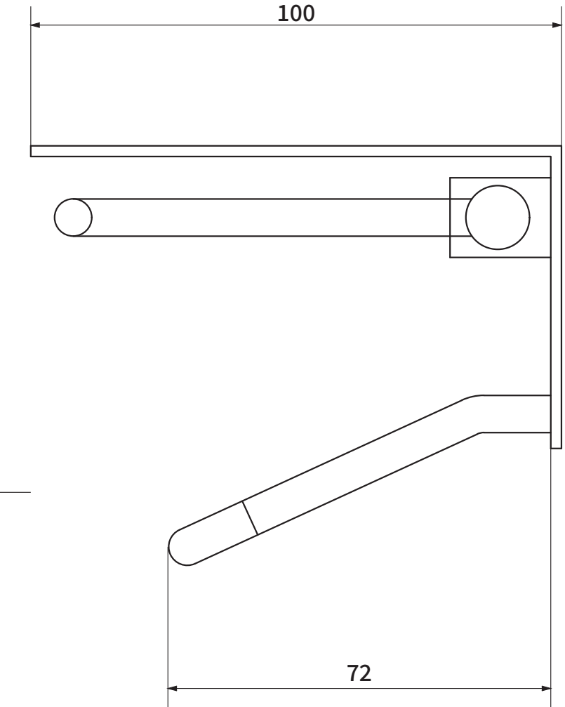
● Side view
