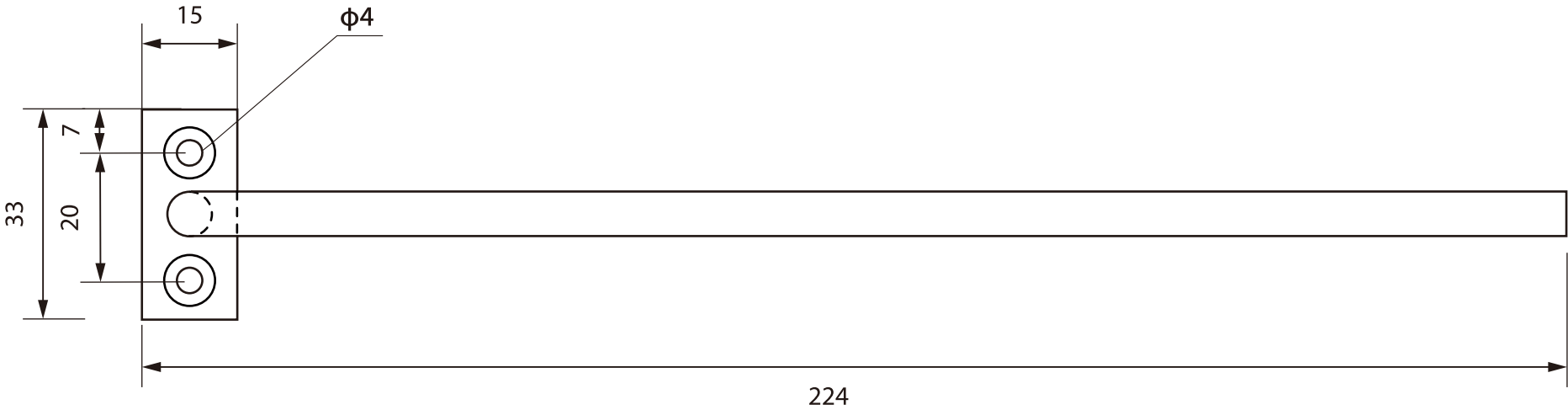
● Front view
