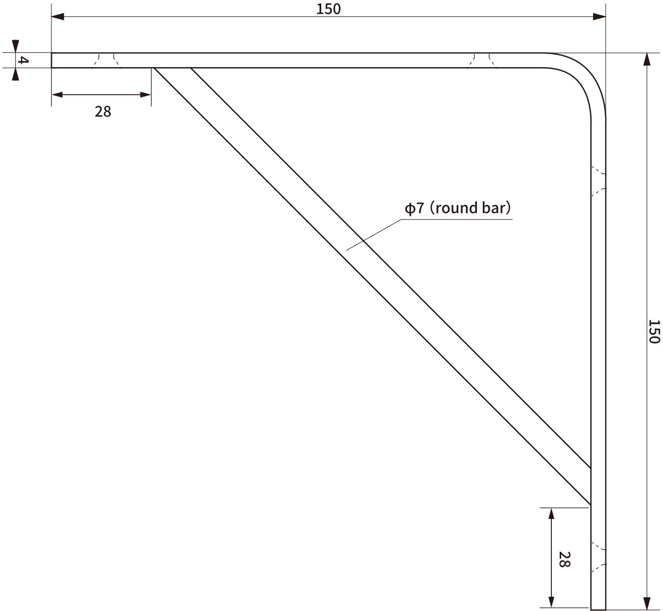
●Side view
