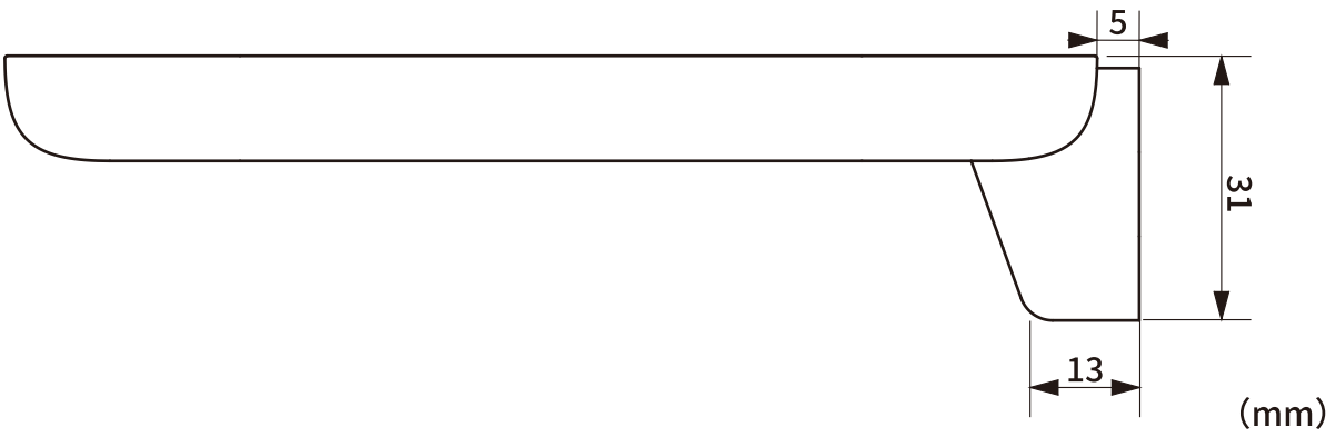
● Side view
