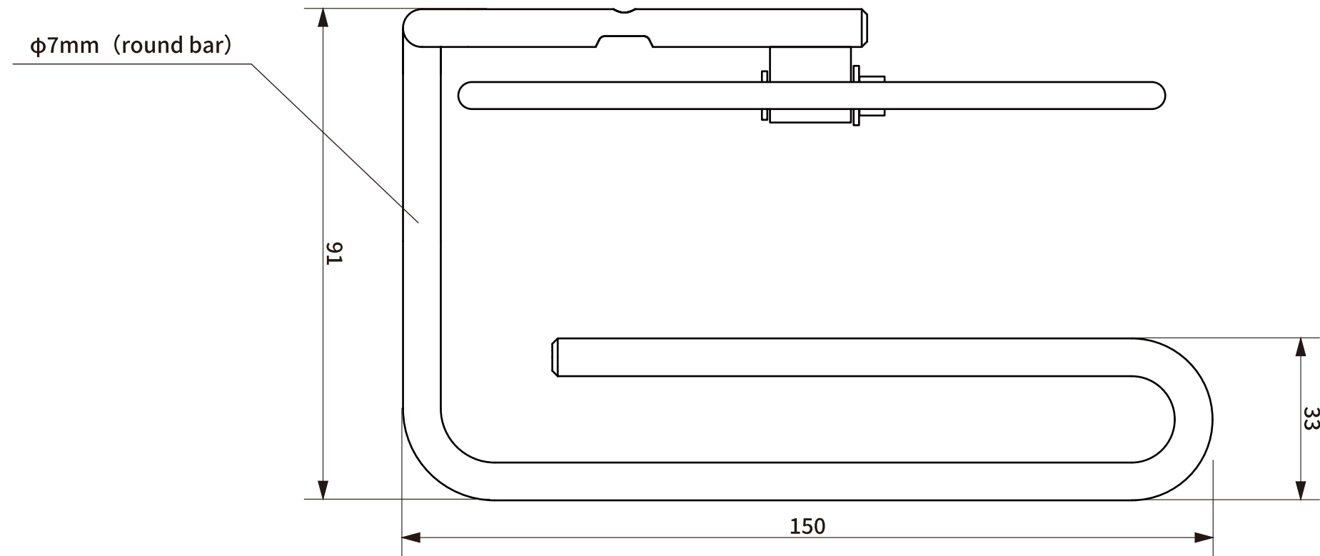
● Front view
