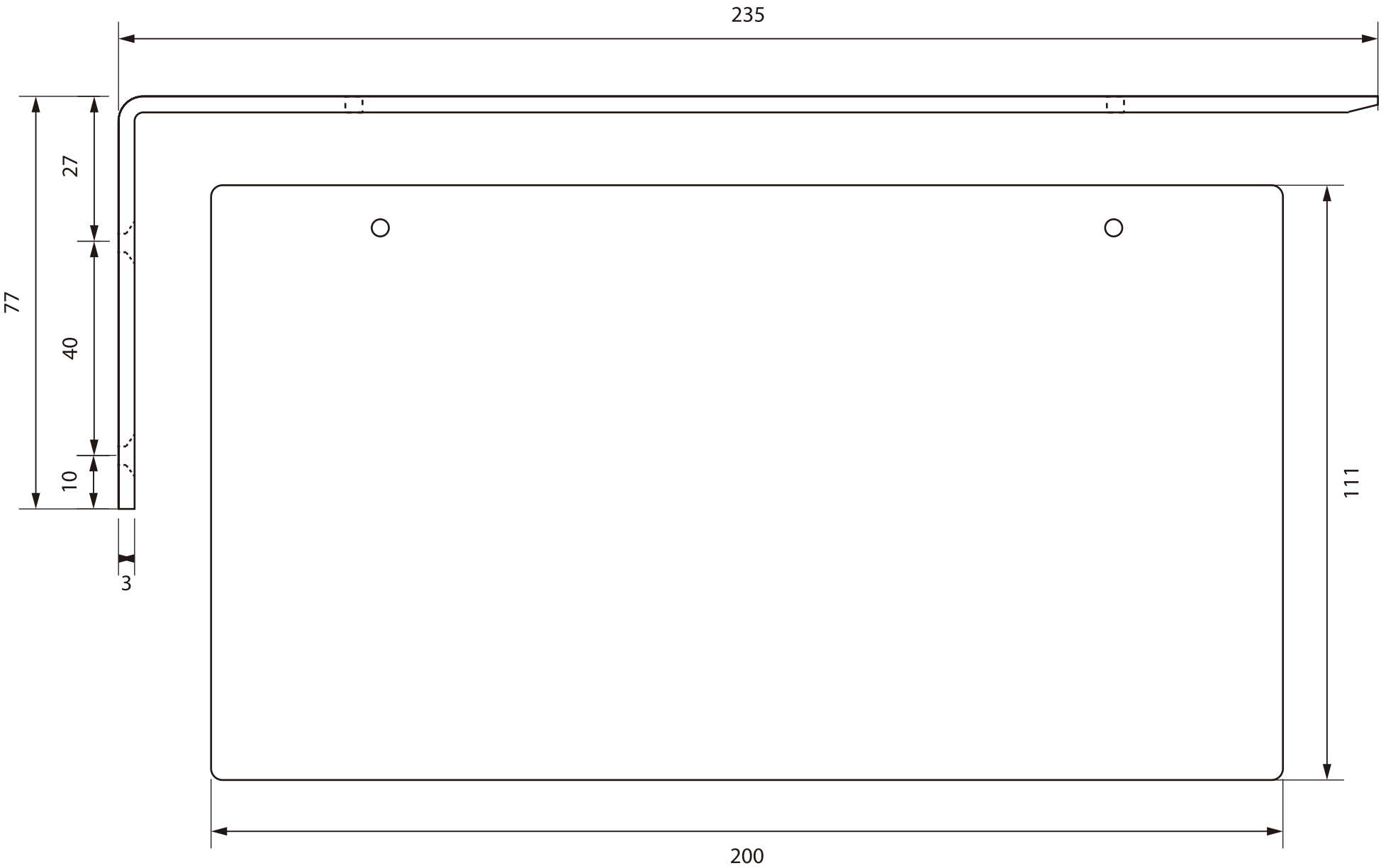
●Front view
