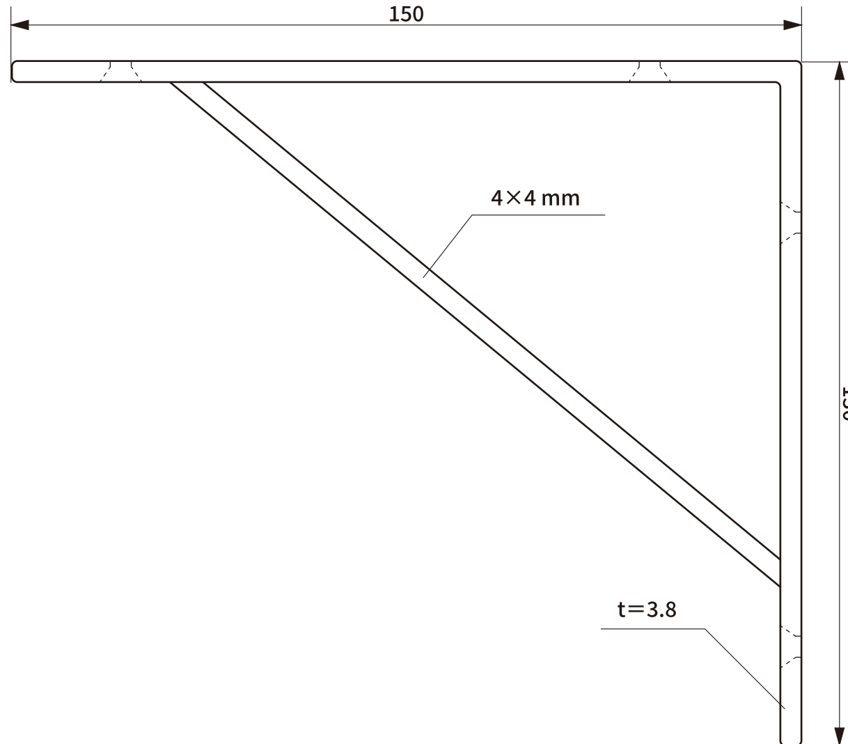
● Side view
